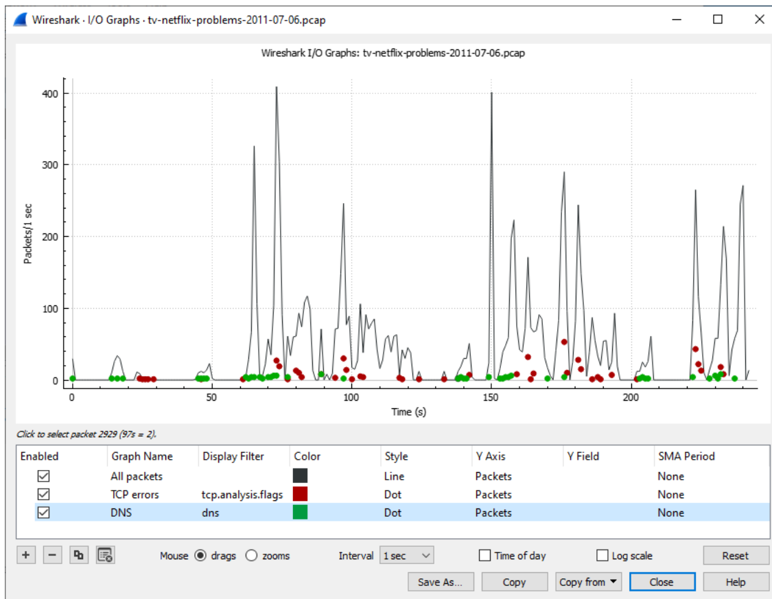
Figure 76. The “I/O Graphs” window
