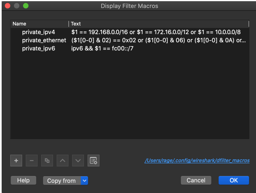
Figure 60. Display Filter Macros window
