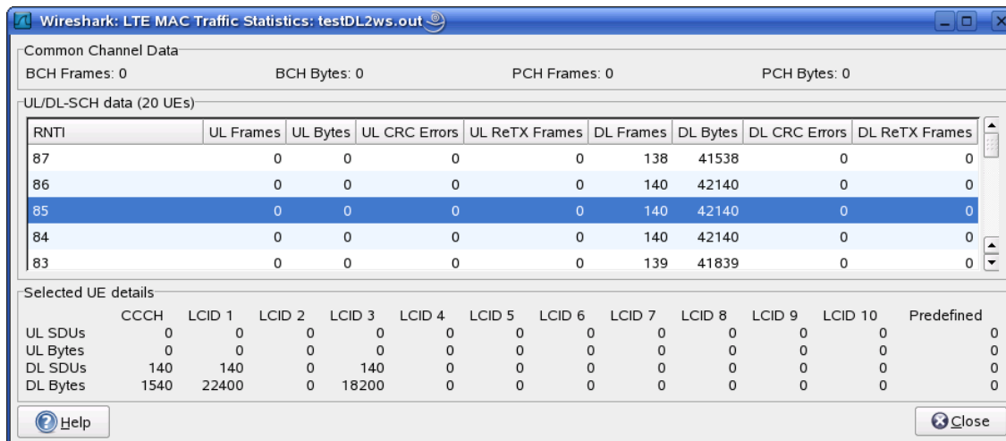
Figure 79. The “LTE MAC Traffic Statistics” window
