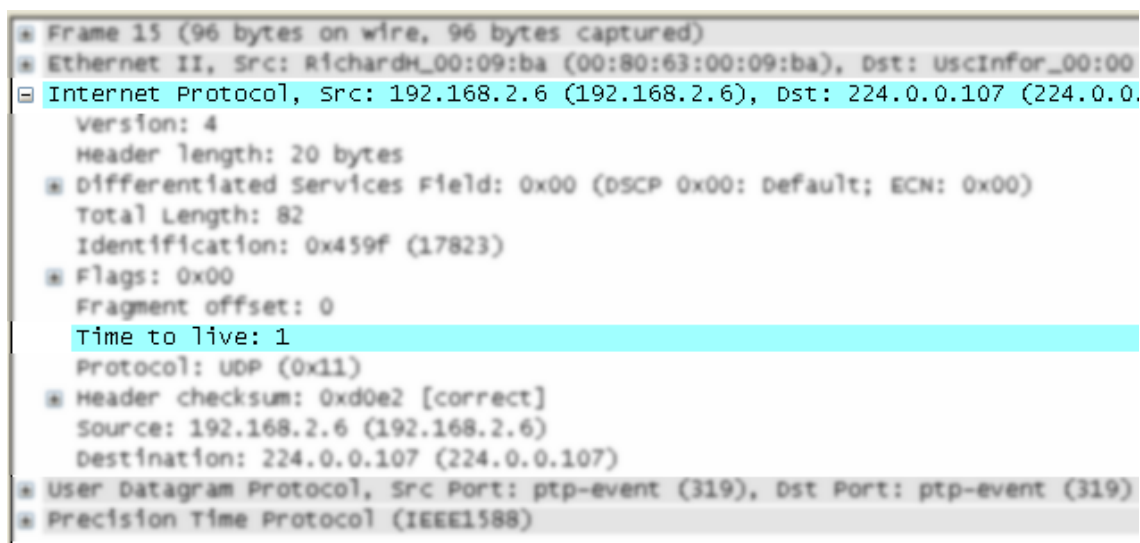
Figure 67. The “Colorized” protocol details tree
