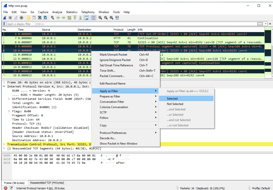
Figure 54. Pop-up menu of the “Packet List” pane
