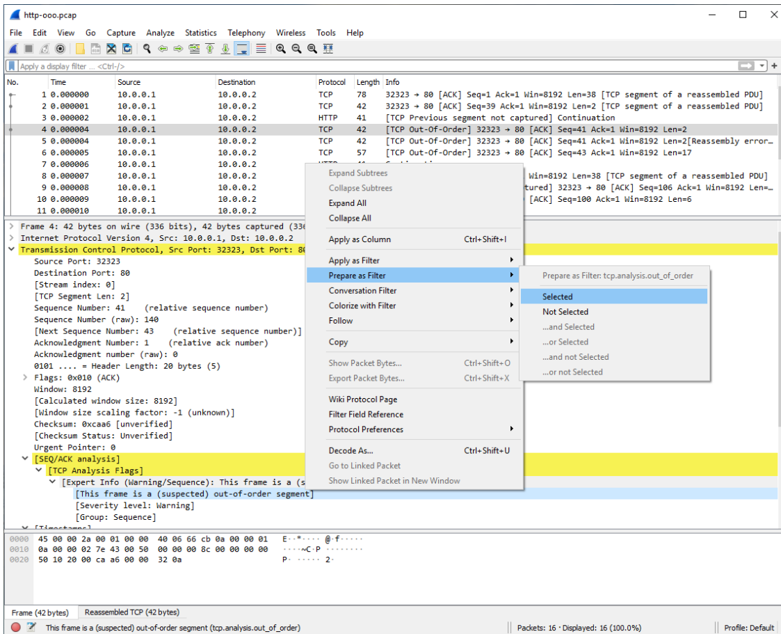
Figure 55. Pop-up menu of the “Packet Details” pane
