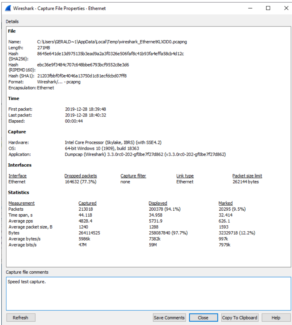
Figure 71. The “Capture File Properties” dialog
