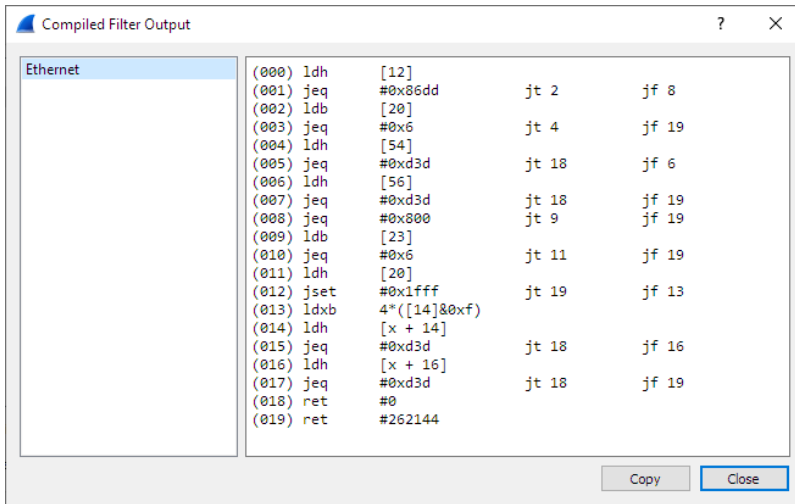
Figure 32. The “Compiled Filter Output” dialog box
