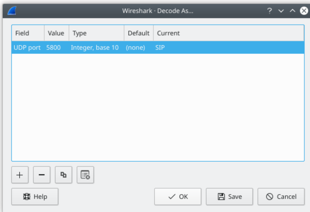
Figure 88. The “Decode As” dialog box
