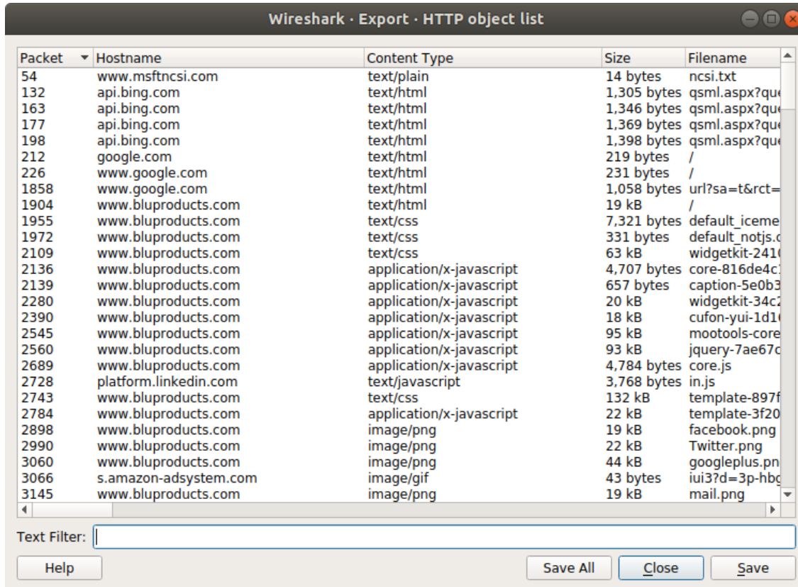
Figure 47. The “Export Objects” dialog box
