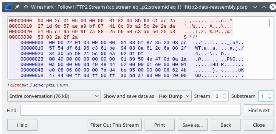
Figure 65. The “Follow HTTP/2 Stream” dialog box
