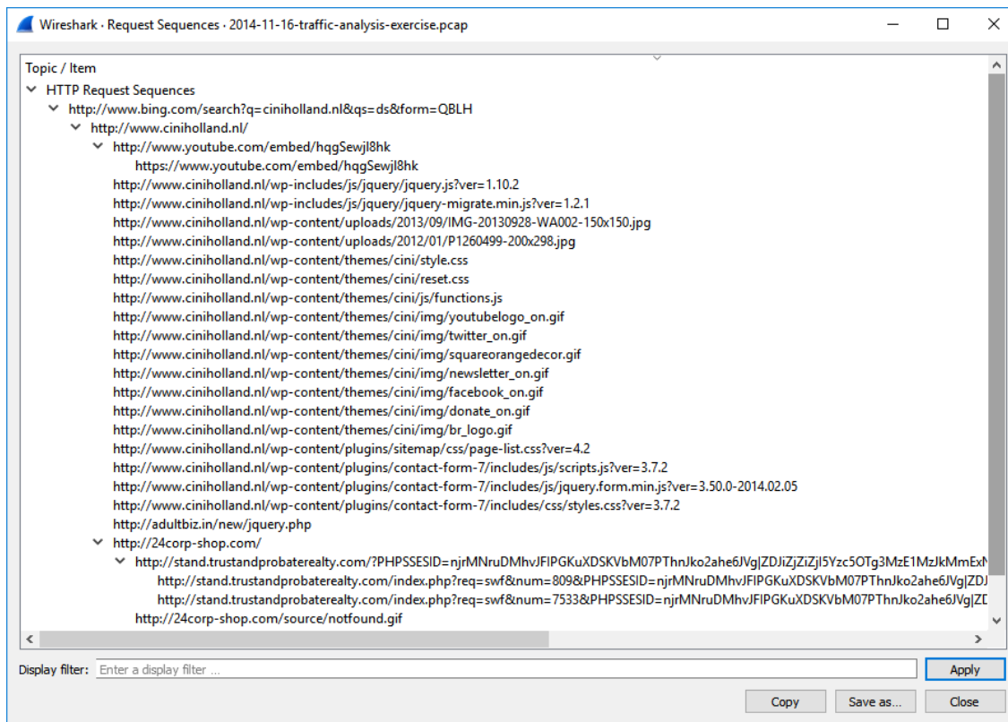
Figure 78. The "HTTP Request Sequences" window
