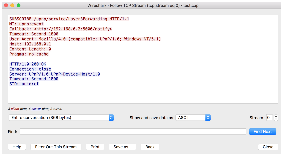
Figure 64. The “Follow TCP Stream” dialog box
