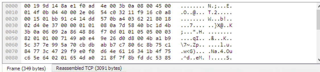
Figure 70. The “Packet Bytes” pane with a reassembled tab
