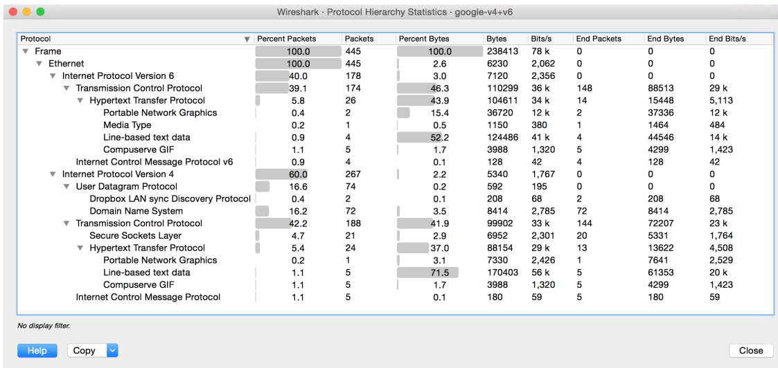
Figure 72. The “Protocol Hierarchy” Window
